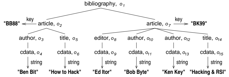
Figure 1: XML document and corresponding syntax tree
